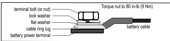
Figure 6 Battery terminal stacking
